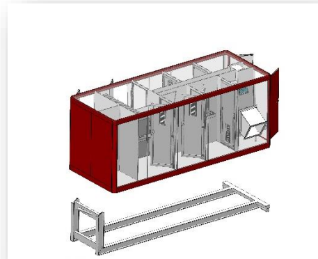
Abrollcontainer (DIN 30722)
